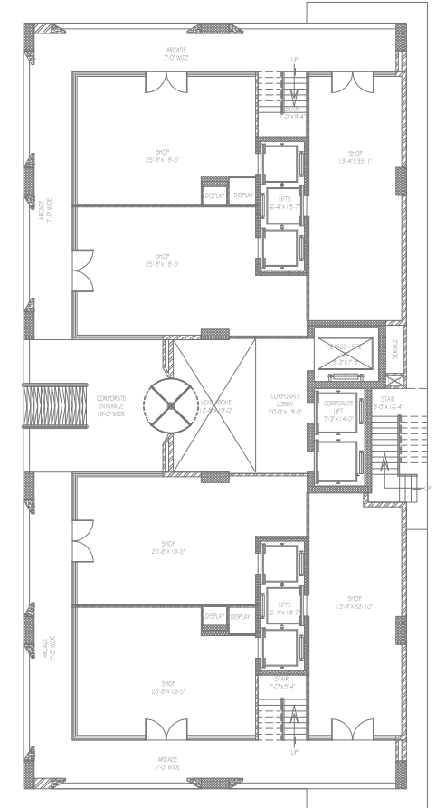
GROUND FLOOR PLAN (SCALE: 1/8" = 1'-0")
